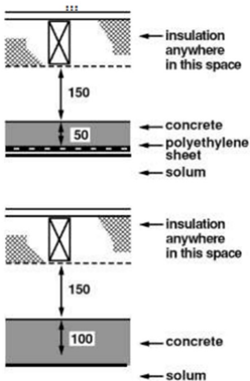
Figure 3.12 Suspended timber floors 2
