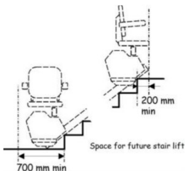
Figure 4.5 Future provision for unassisted access
