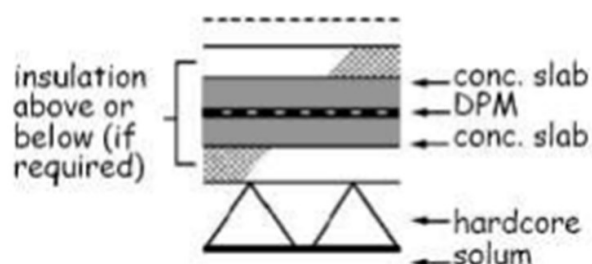
Figure 3.9 Ground supported concrete floors 3
