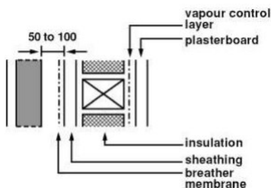
Figure 3.22 Wall constructions - Type A
