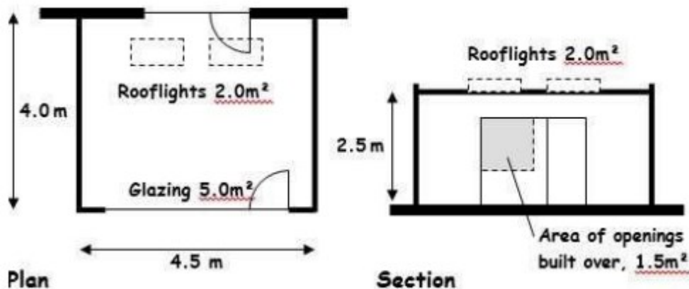
Figure 6.2 Single Storey extension
