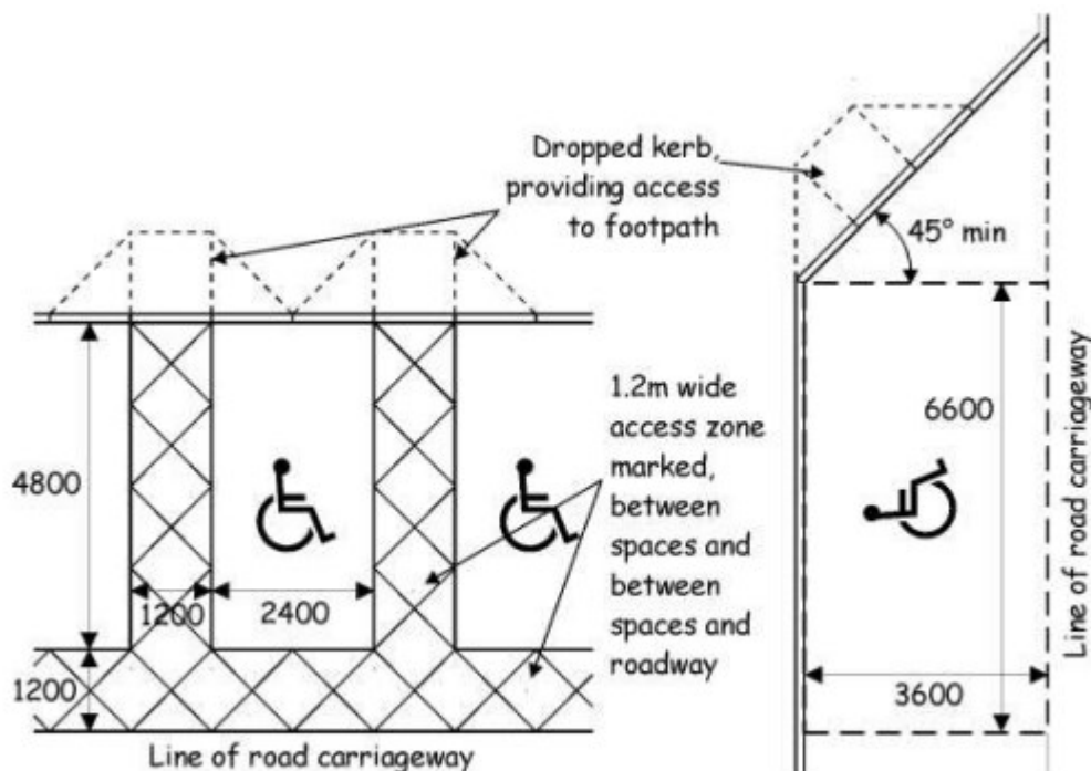
Figure 4.1 Off- and on-street accessible car parking
