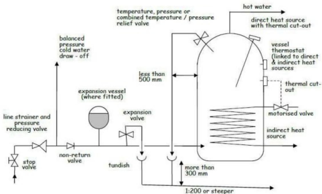
Figure 4.12 Unvented hot water storage system – indirect example
