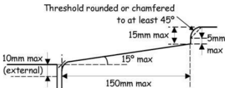
Figure 4.3 Generic threshold profile
