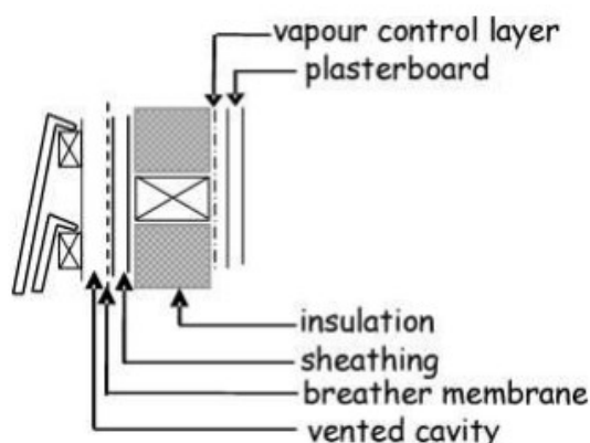
Figure 3.23 Wall constructions - Type B
