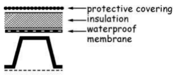
Figure 3.30 Roof constructions - Type F
