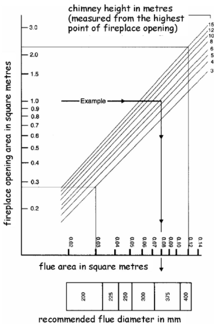
Figure 3.58 Fireplace opening areas
