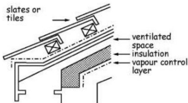
Figure 3.41 Roof type B insulation on a sloping ceiling
