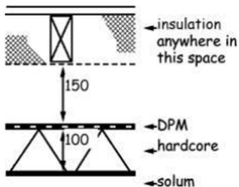
Figure 3.11 Suspended timber floors 1
