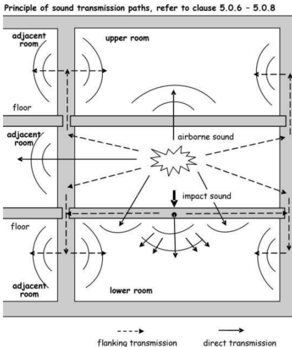
Figure 5.1 principle of sound transmission paths
