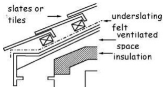
Figure 3.31 Roof constructions -Type A
