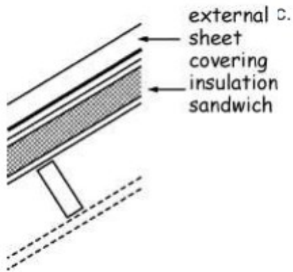
Figure 3.34 Roof constructions - Type D
