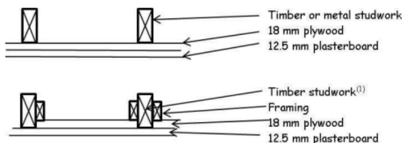
Figure 3.39 Typical Robust wall construction
