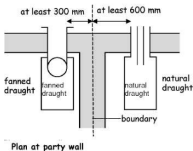
Figure 3.65 Separation between a boundary and terminal at right angles
