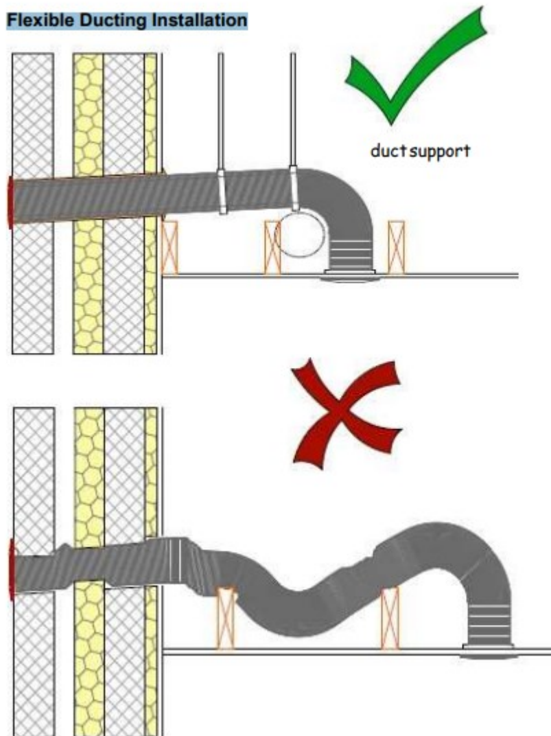
Figure 3.67 Flexible Ducting Installation
