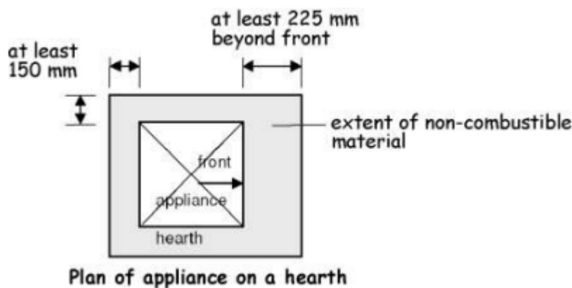
Figure 3.53 Plan of appliance on a hearth (gas-fired)
