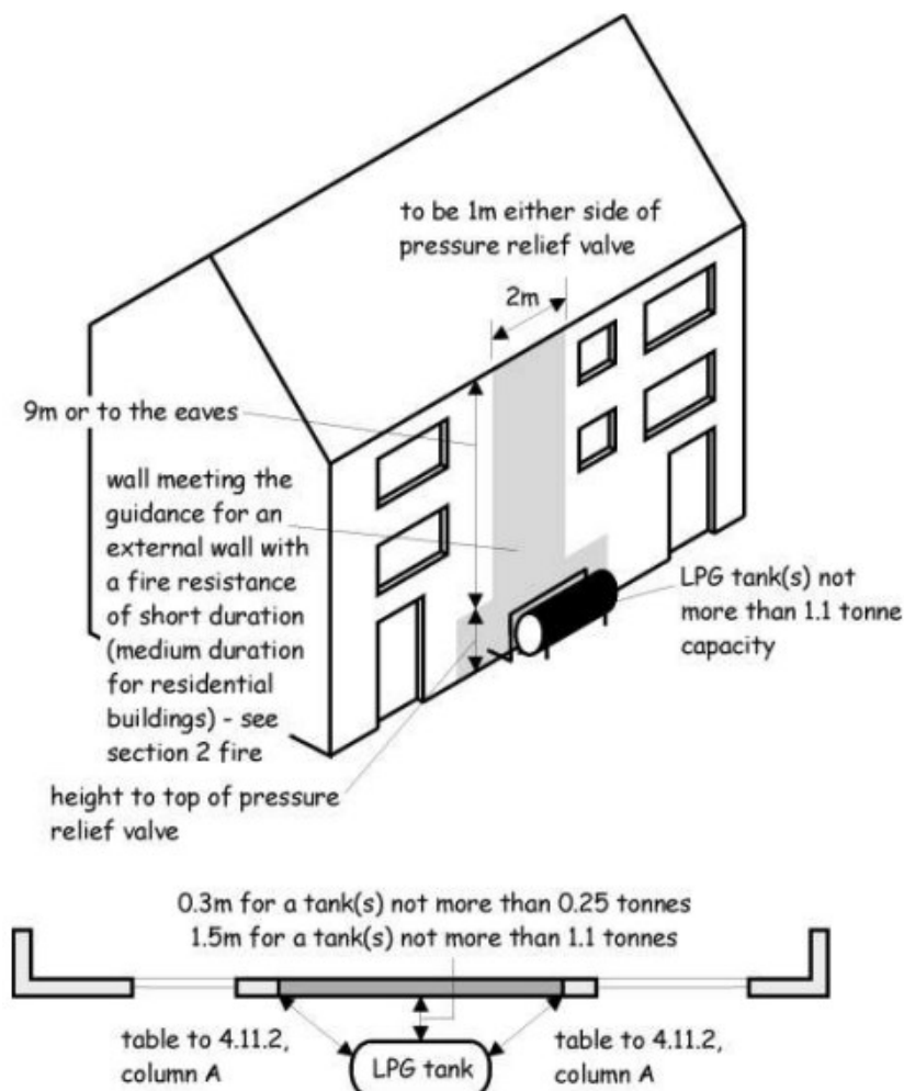
Figure 4.14 Small LPG tank close to a building
