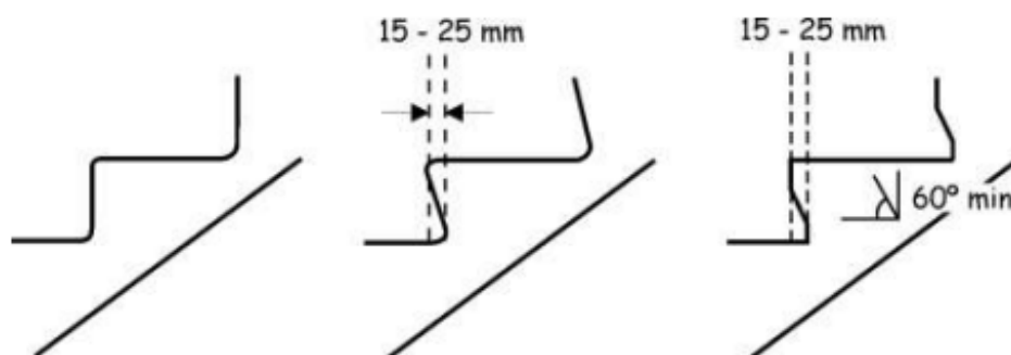
Figure 4.7 Step profile examples
