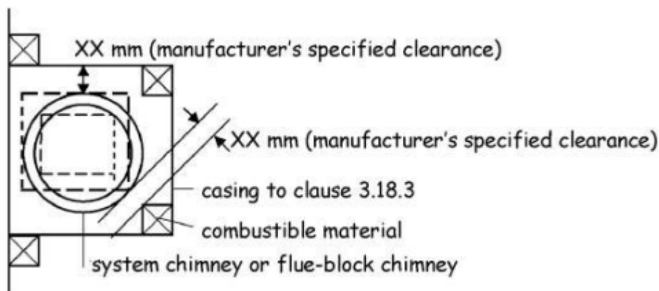
Figure 3.45 Plan of casing round a factory-made chimney
