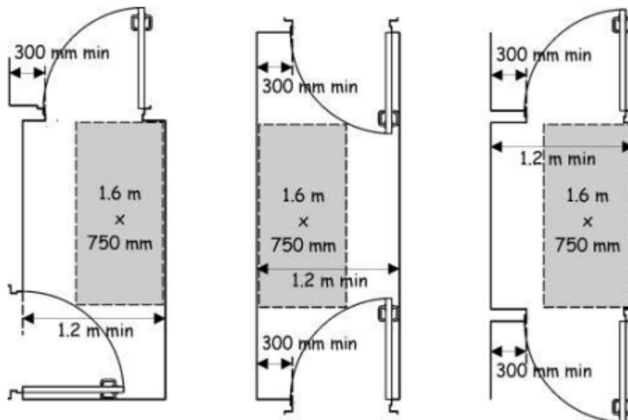
Figure 4.4 Accessible lobby dimensions
