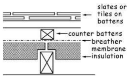
Figure 3.33 Roof constructions -Type C
