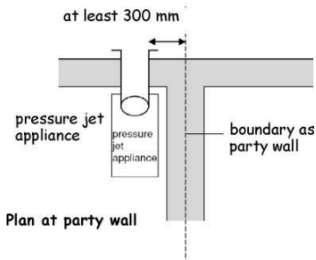
Figure 3.63 Separation between a boundary and terminal at right angles
