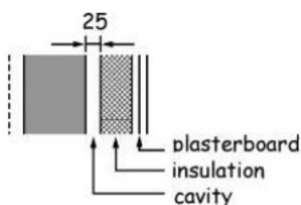
Figure 3.17 Wall constructions -Type A
