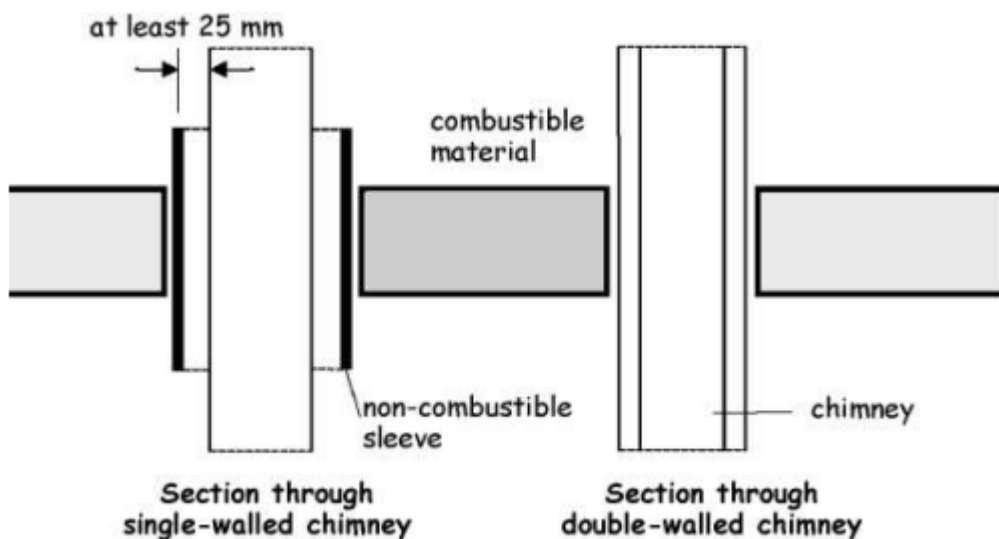
Figure 3.46 Section through single-walled Chimney (vertical)
