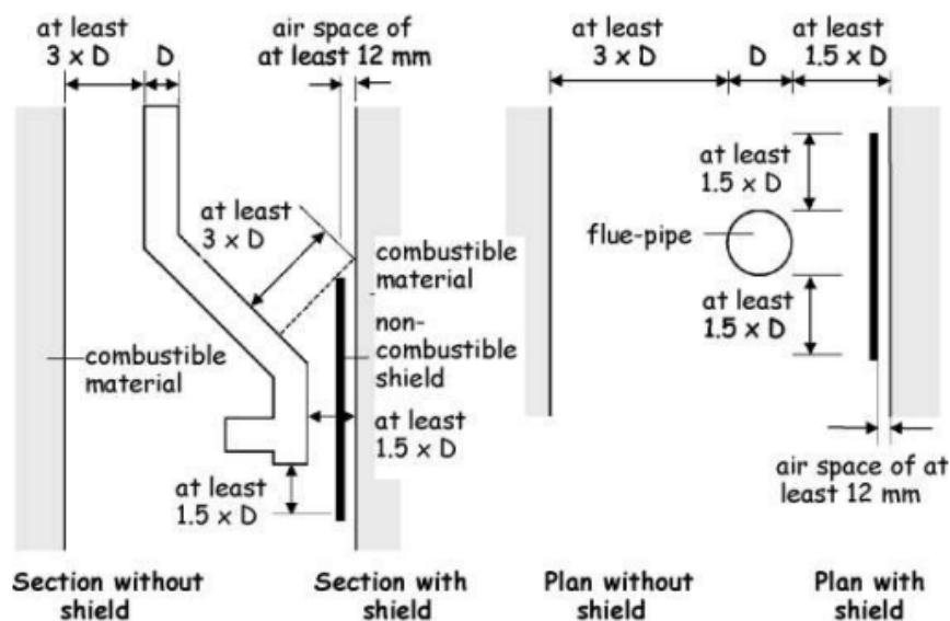
Figure 3.48 Relationship of flue-pipes to combustible material
