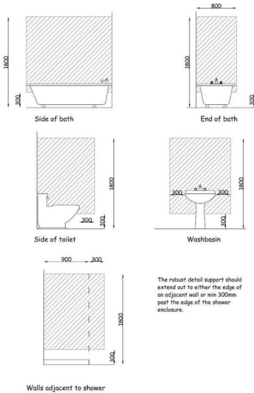
Figure 3.38 Robust wall construction
