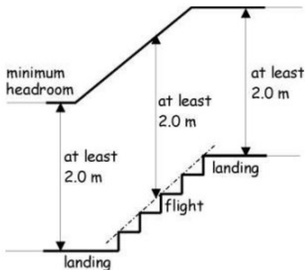
Figure 4.11 Headroom on stairs and ramps
