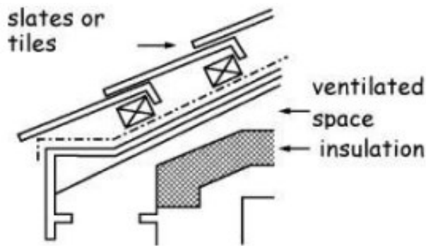
Figure 3.40 Roof Type A insulation on a level ceiling
