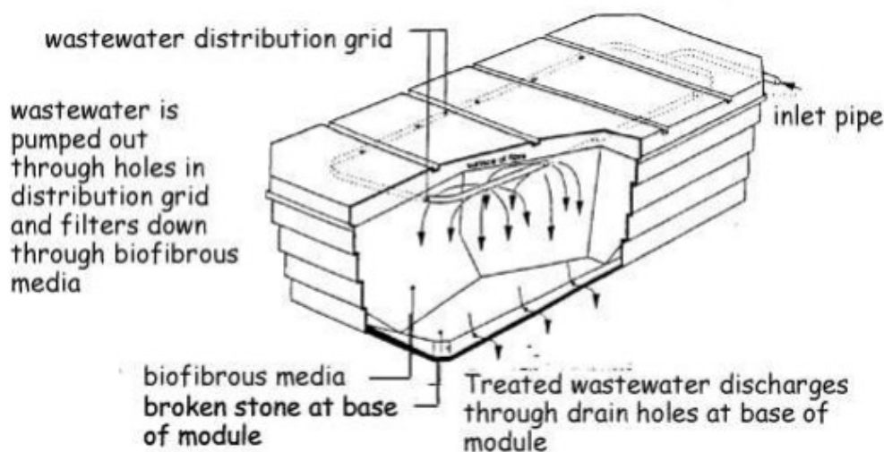
Figure 3.16 Typical proprietary filtration system
