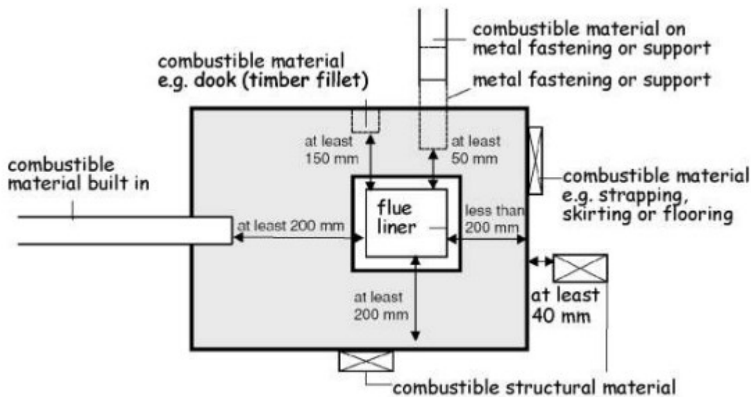
Figure 3.44 Plan view of masonry chimney
