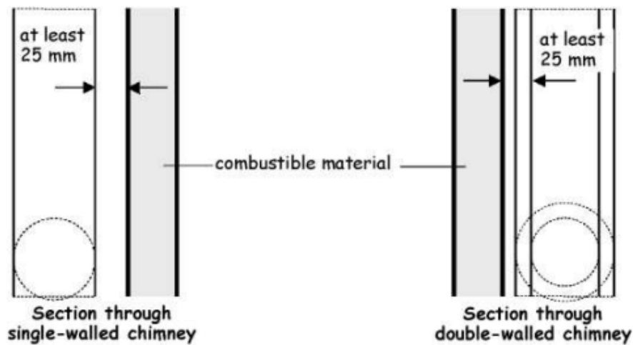
Figure 3.47 Section through double-walled Chimney (horizontal)
