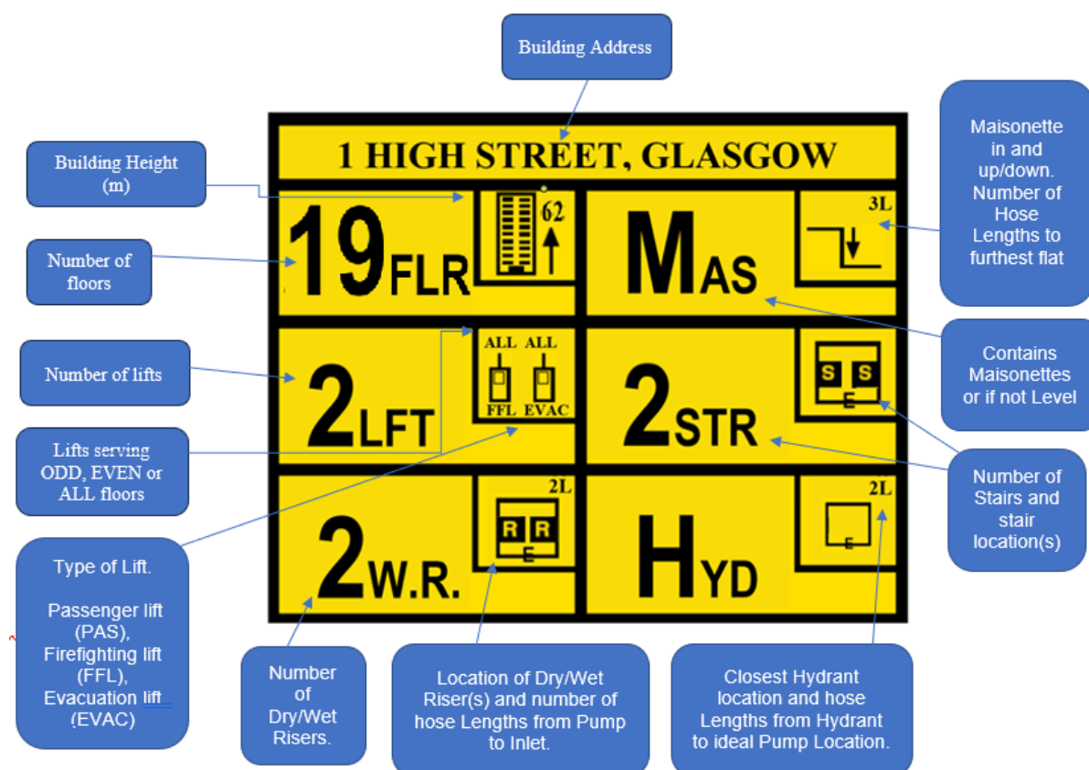
Figure 2.12 Typical Premises Information Plate – Required information
