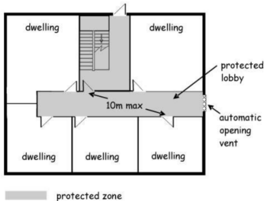
Figure 2.5 Upper Floor - Two Escape Routes
