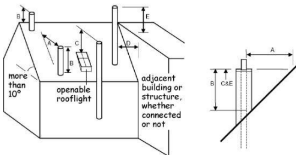
Figure 3.60 Solid fuel - flue outlets
