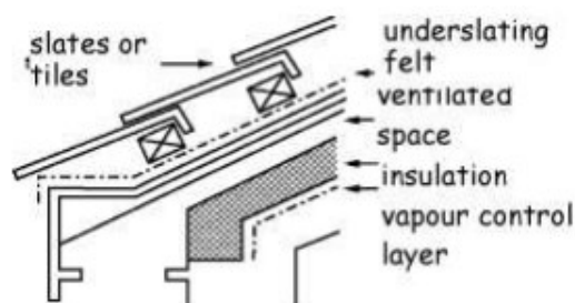
Figure 3.32 Roof constructions -Type B
