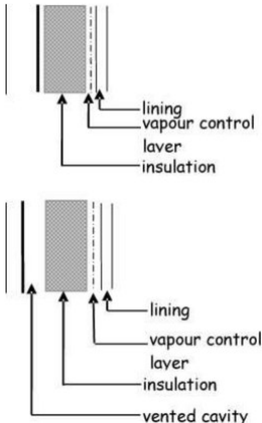
Figure 3.24 Wall constructions - Type C
