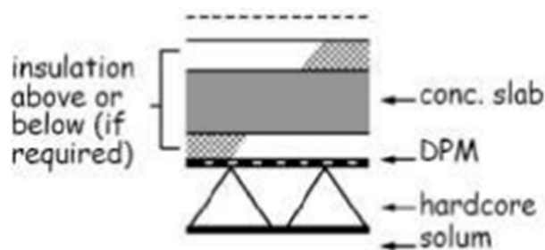
Figure 3.8 Ground supported concrete floors 2
