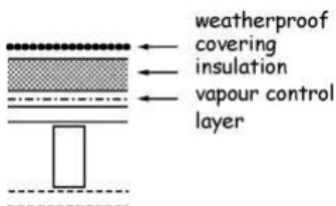
Figure 3.27 Roof constructions – Type C
