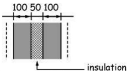
Figure 3.20 Wall constructions -Type B
