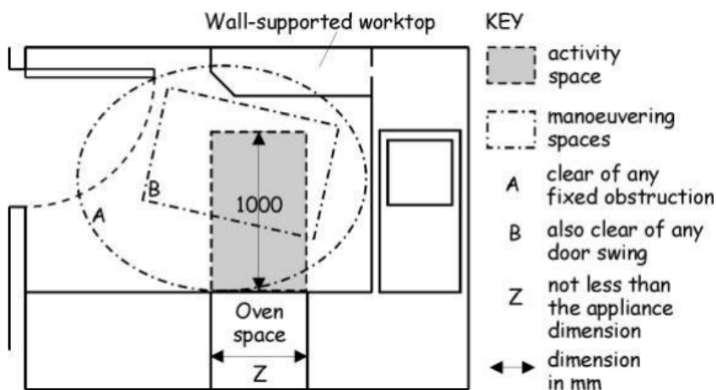
Figure 3.36 Space provision within a kitchen
