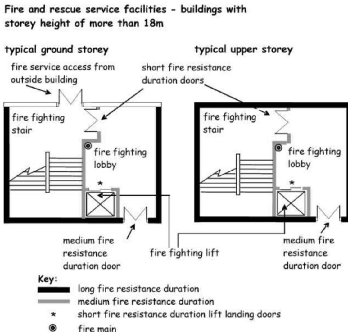
Figure 2.9 Building with a storey height more than 18 m
