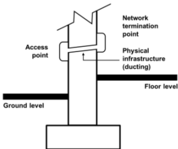
Figure 4.15 In-building physical infrastructure serving a single dwelling
