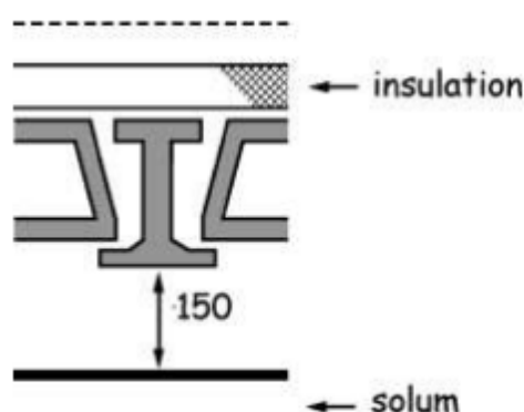
Figure 3.10 Suspended concrete floors
