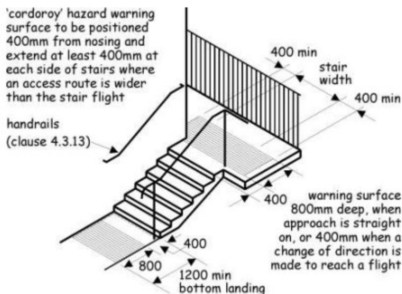
Figure 4.8 Use of corduroy tactile paving
