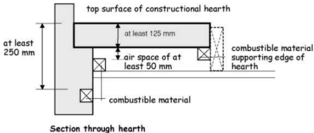
Figure 3.56 Section through hearth
