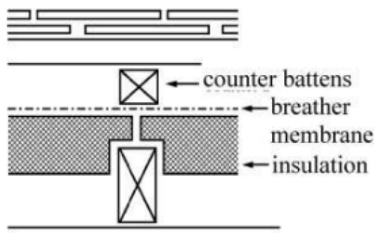
Figure 3.42 Roof type B insulation on a sloping ceiling
