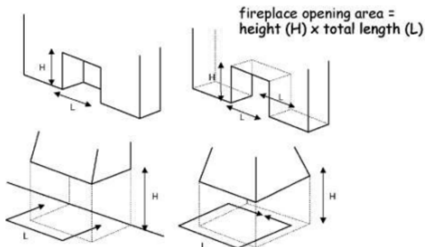
Figure 3.58 Fireplace opening areas
