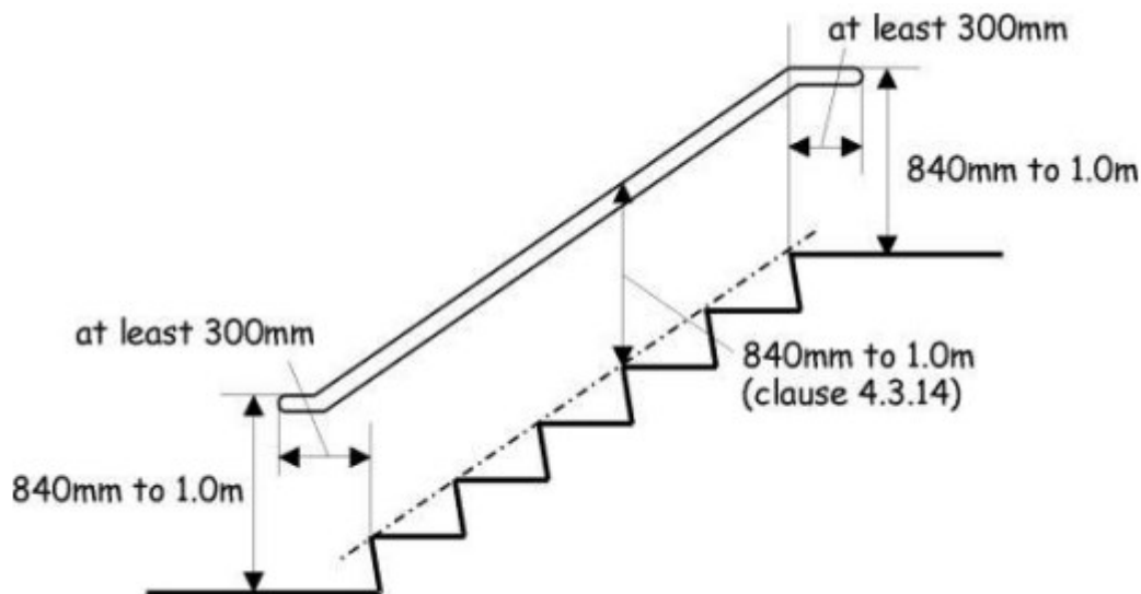
Figure 4.10 Handrails to stairs and ramps
