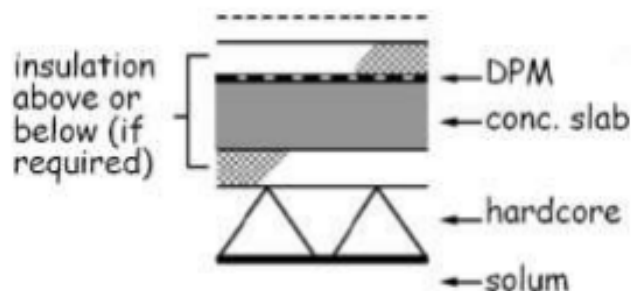
Figure 3.7 Ground supported concrete floors 1
