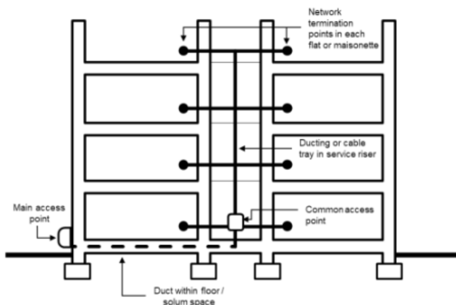
Figure 4.16 In-building infrastructure serving flats or maisonettes
