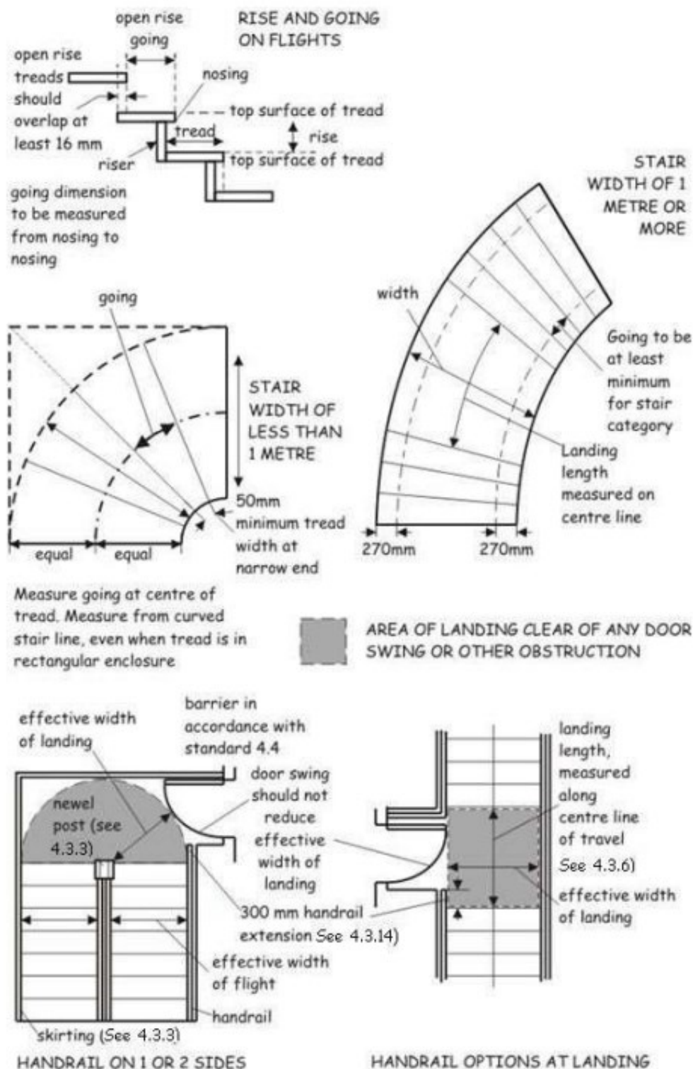
Figure 4.6 Measurement for stairs
