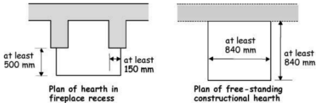
Figure 3.49 Hearth construction
