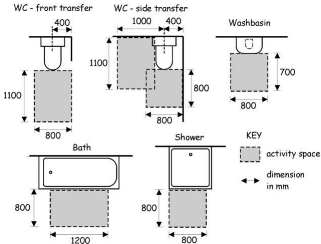
Figure 3.37 Activity spaces for accessible sanitary facilities
