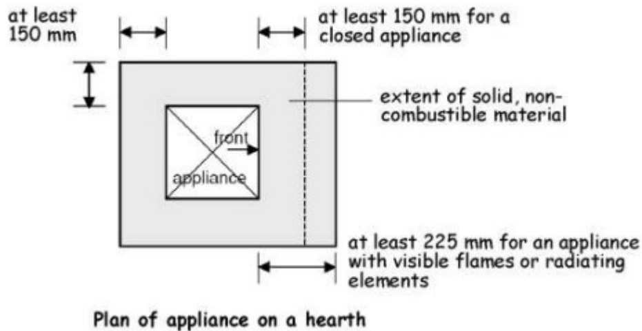
Figure 3.52 Plan of appliance on a hearth (oil-firing)
