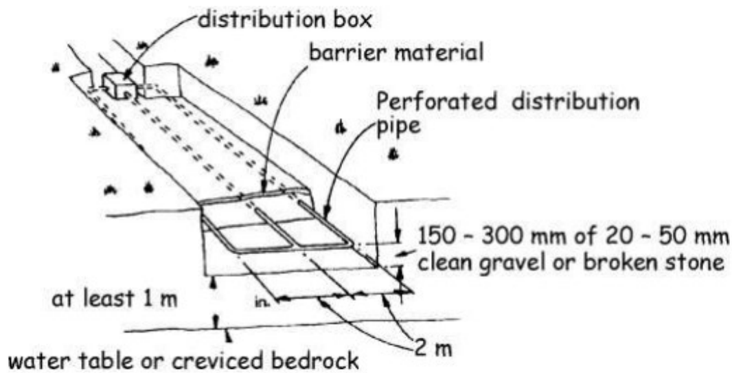
Figure 3.15 Piped infiltration bed system
