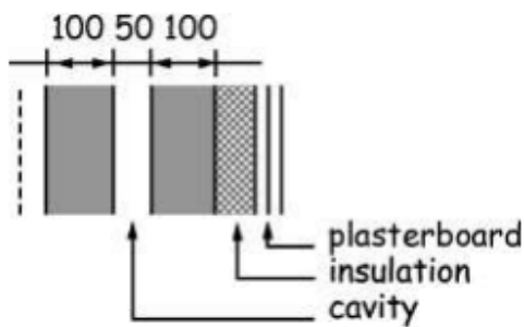
Figure 3.19 Wall constructions - Type A
