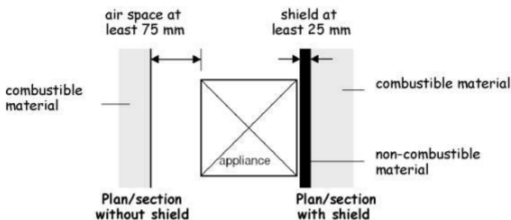
Figure 3.54 Plan of appliance on a hearth (separation)
